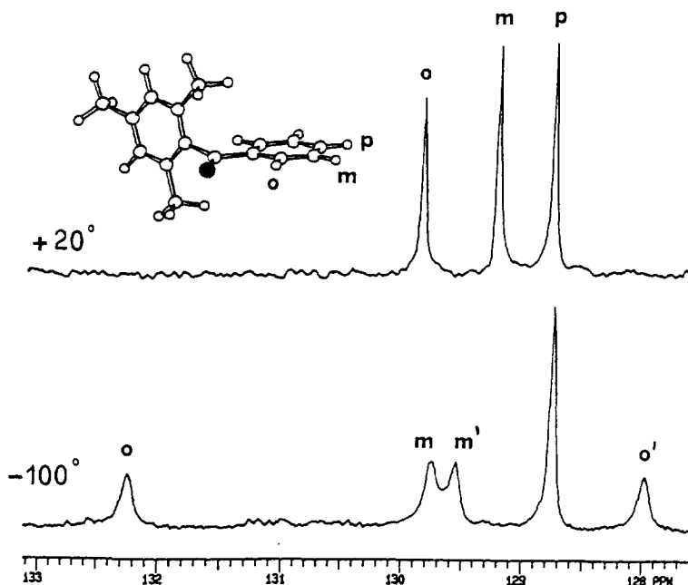
Fig 2. Top : Room Temperature ^{13}C Lines (75.5 MHz in CD_2Cl_2 ) of the ortho , para and meta Carbons of the Phenyl Group of 1f . Bottom : the Same Spectral Region at -100^\circ Displays a Large Splitting for the ortho and a Smaller one for the meta Carbons, due to the Restricted Ph-CO Rotation.
